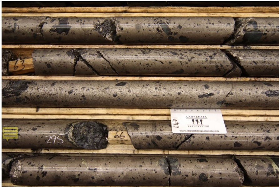
Figure 7: Zoomed in core photo of GRL-22-60 showing the massive sulphides (News Release February 16, 2023)
