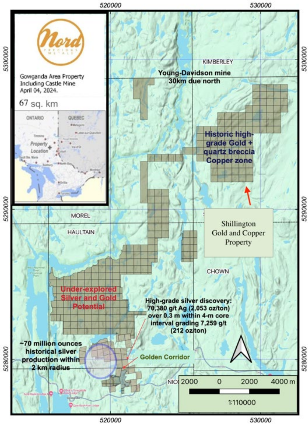
Figure 1: Nord Precious Metals - Castle Property
