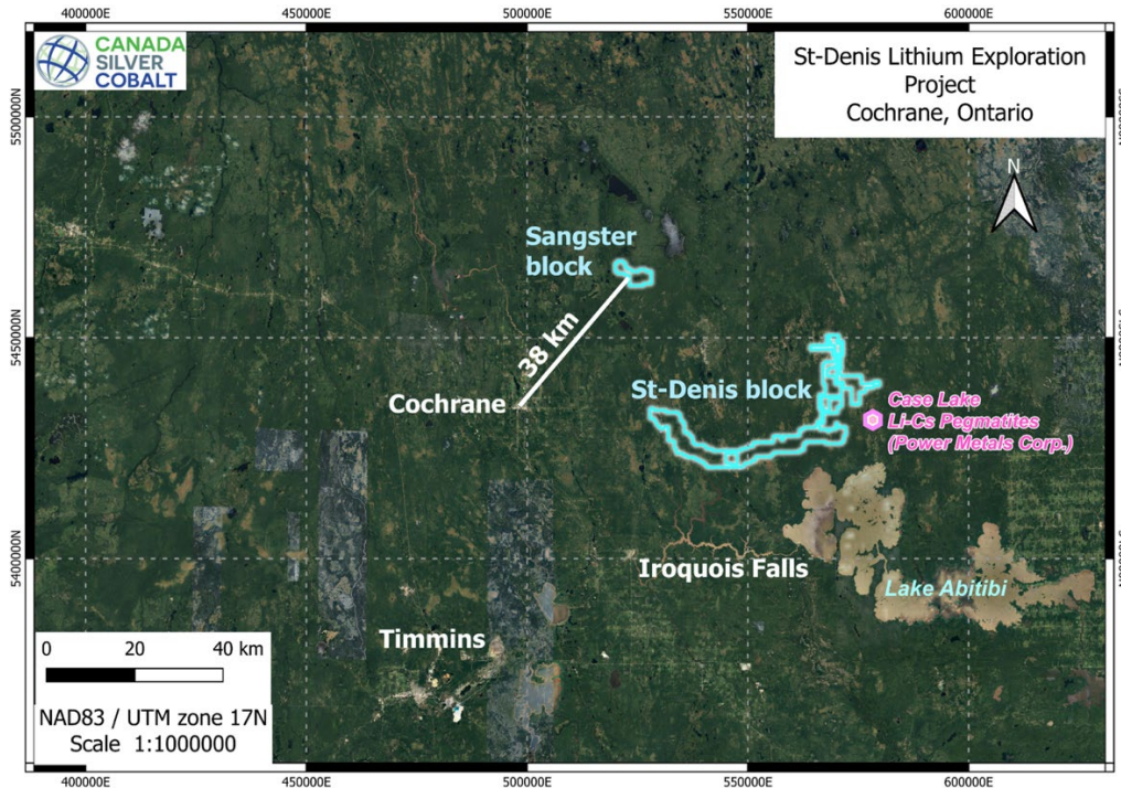
Figure 8: Location of the St-Denis Project and Sangster claim block
