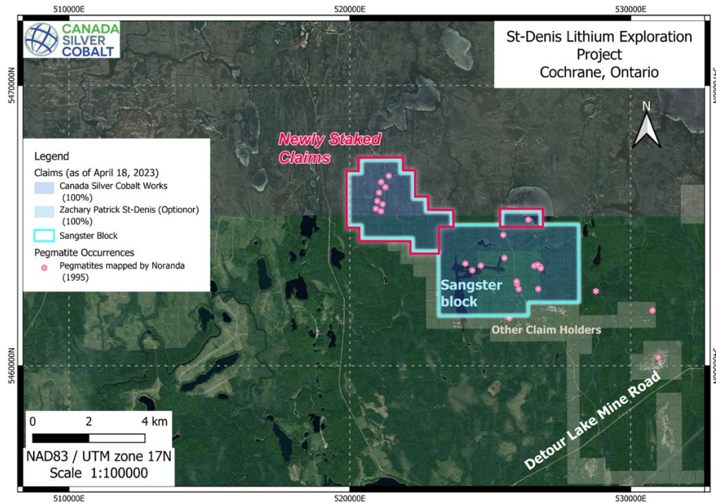
Figure 9: Location of expanded claim staking by Nord Precious Metals
