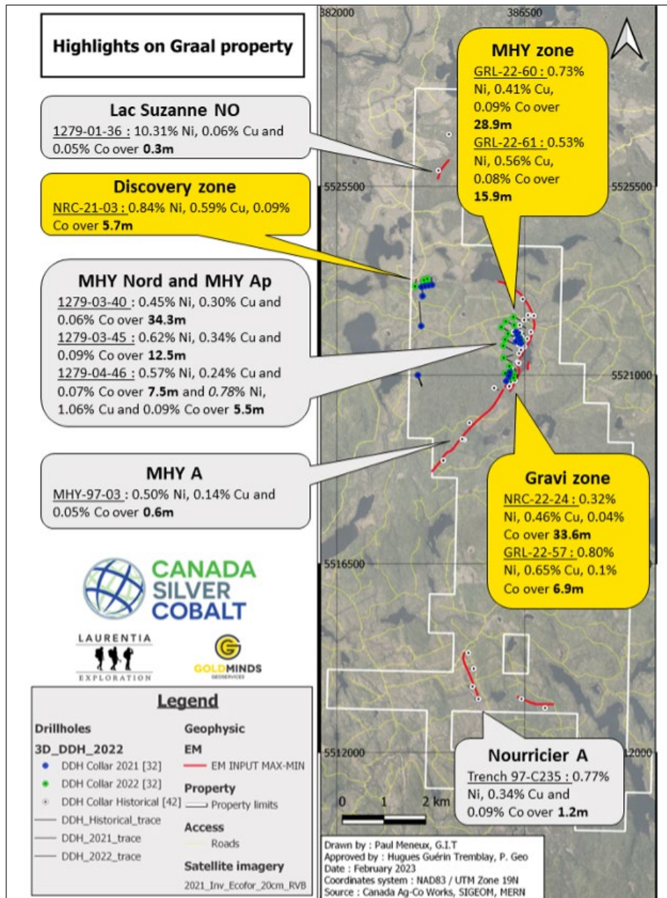
Figure 5: Showing location of select assay highlights from historic drilling, Phase 1 and Phase 2
